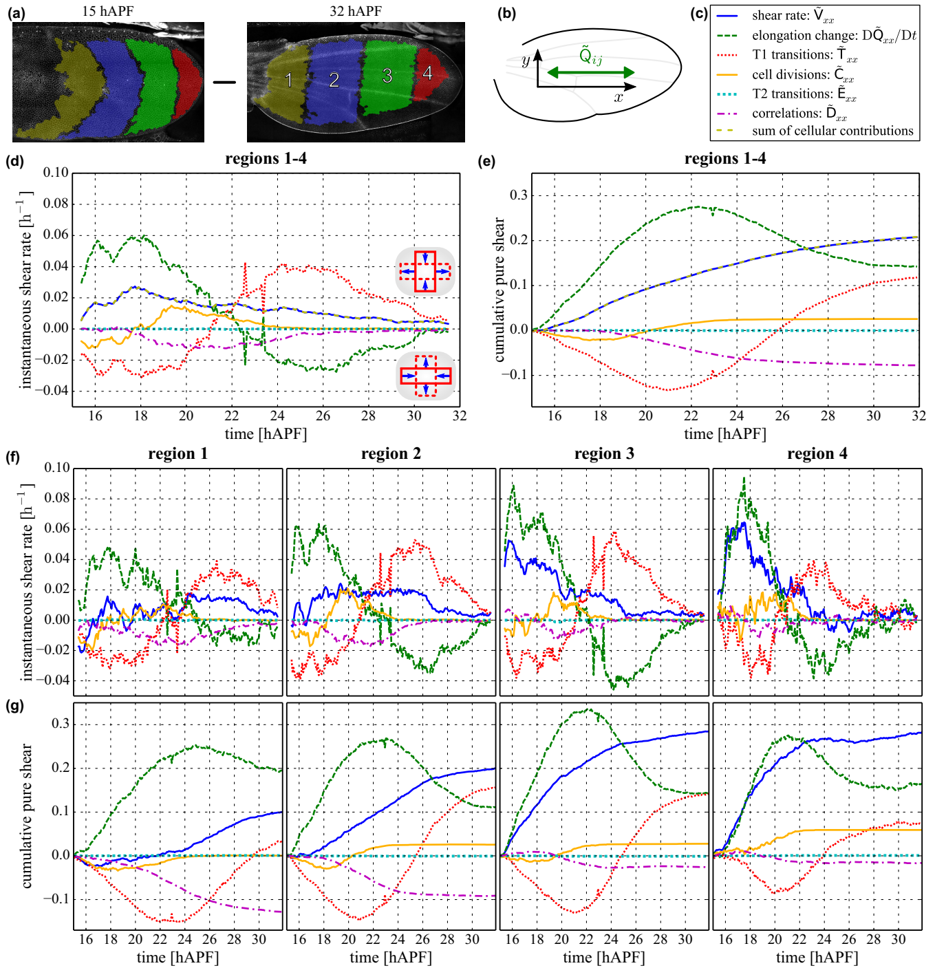
FIG. 11. Contributions to tissue shear as a function of time during pupal development of the fly wing. Shown are the data for one wing. (a) The fly wing undergoes complex tissue remodeling, which we recorded between 15 and 32 hAPF. The colored areas mark regions of tissue in which all cells were tracked during this time interval. (b) Schematic representation of the coordinate system used to describe tissue deformations. The x axis points towards the tip of the wing and is aligned parallel to the axis of cell elongation averaged within the interval between 24 and 32 hAPF and over all four regions. The average cell elongation computed for a single region deviates at most by 5^\circ from this x axis. (c) Legend specifying different contributions to tissue shear. (d) Cellular contributions to shear and total shear rate averaged over regions 1–4 in (a) as a function of time. Plotted are the projections of the tensors on the x axis, for example, the component \tilde{V}_{xx} of the tissue shear rate. (e) Cumulative tissue shear and cellular contributions, projected on the x axis. (f), (g) Same plots as in (d) and (e), but for the subregions 1 to 4 indicated in (a). In (d)–(g), data were averaged over 10 subsequent interframe intervals.
