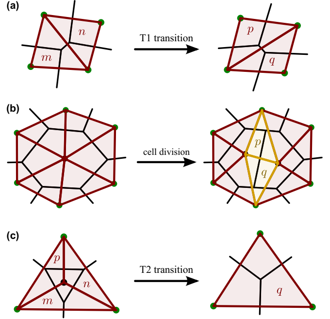
FIG. 7. Effects of a single topological transition on the triangulation. (a) A T1 transition removes two triangles ( m and n ) and creates two new ones ( p and q ). (b) A cell division creates two triangles ( p and q , yellow). All other triangles shown (red) change their shape instantaneously. (c) A T2 transition removes three triangles ( m , n , p ) and creates a new one ( q ).
