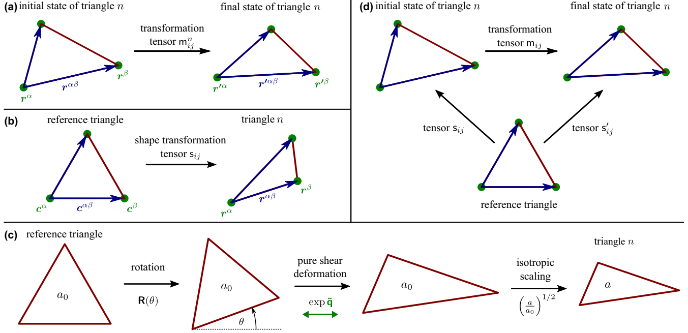
FIG. 4. Characterization of triangle deformation and shape. (a) Deformation of a triangle n from an initial state to a final state. The deformation is characterized by the linear transformation tensor m_{ij}^n mapping the initial side vectors of the triangle to the final side vectors (blue arrows). (b) The shape of a triangle n in a given state is characterized by the tensor S_{ij} . Tensor S_{ij} maps the side vectors of a virtual equilateral reference triangle to the side vectors of triangle n (blue arrows). (c) Shape properties of a triangle n . The transformation tensor S_{ij} is decomposed into a counterclockwise rotation by the triangle orientation angle \theta , a pure shear deformation characterized by the triangle elongation tensor \tilde{q}_{ij} , and an isotropic rescaling to match the actual triangle area a . (d) Connection between triangle shape and triangle deformation. A triangle deforms from an initial state to a final state. Deformation, initial state, and final state are characterized by the tensors m_{ij} , S_{ij} , and S'_{ij} , respectively.
