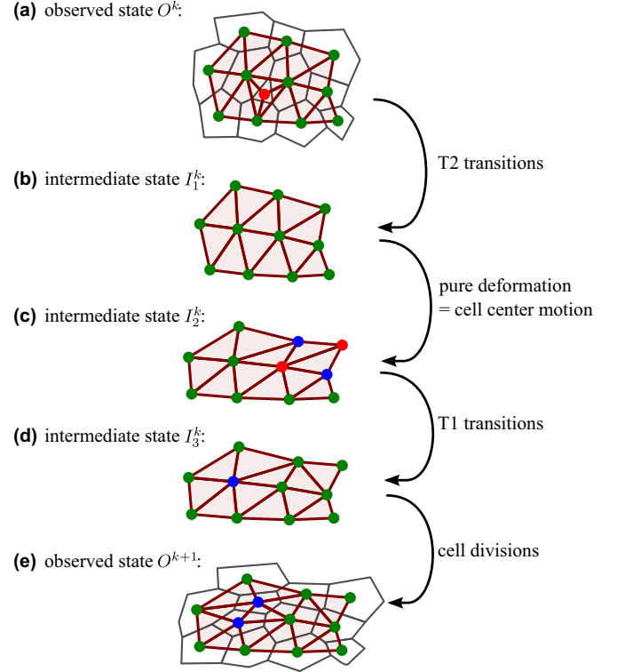
FIG. 17. Illustration of the virtual intermediate states I_1^k , I_2^k , and I_3^k introduced between two observed states O^k and O^{k+1} .
