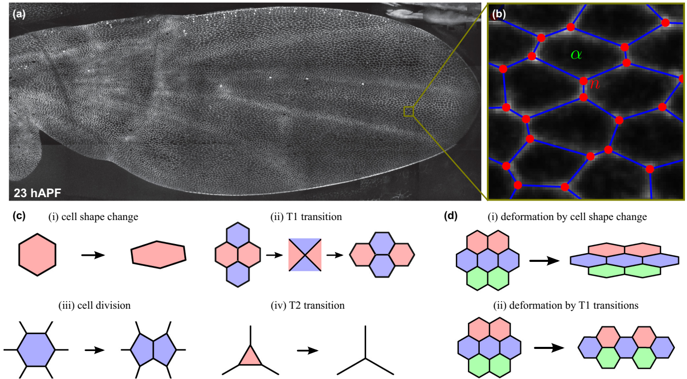
FIG. 1. (a) The developing fly wing is an important model system to study epithelial morphogenesis. This panel shows the wing blade at the developmental time of 23 h after puparium formation (hAPF). (b) Magnified region of membrane-stained wing tissue overlaid with the corresponding polygonal network. Cells are represented by polygons (green), cell-cell interfaces correspond to polygon edges (blue), and polygon corners correspond to vertices (red). (c) We consider four kinds of cell-scale processes. (d) Two examples for pure shear of a piece of cellular material: (i) pure shear by cell shape change and (ii) pure shear by T1 transitions. Colors in panels (c) and (d) indicate cell identities.
