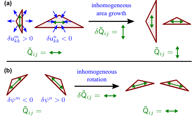
FIG. 5. Correlation contributions to pure shear. (a) Inhomogeneous isotropic expansion that is correlated with elongation creates a change in the average elongation \tilde{\mathbf{Q}}_{ij} , which is due to the area weighting in the definition of \tilde{\mathbf{Q}}_{ij} . This contribution to the time derivative of \tilde{\mathbf{Q}}_{ij} is compensated for by the growth correlation term in \delta\tilde{\mathbf{K}}_{ij} . (b) Inhomogeneous rotation that is correlated with elongation creates a change in the average elongation \tilde{\mathbf{Q}}_{ij} . This contribution to the time derivative of \tilde{\mathbf{Q}}_{ij} is compensated for by the rotational correlation term in \delta\tilde{\mathbf{K}}_{ij} .
