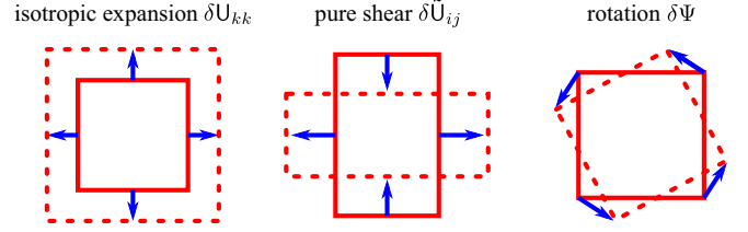
FIG. 3. Infinitesimal displacement gradients \delta \mathbf{U}_{ij} can be decomposed into trace \delta \mathbf{U}_{kk} describing isotropic expansion, symmetric, traceless part \delta \tilde{\mathbf{U}}_{ij} describing pure shear, and antisymmetric part \delta \Psi describing rotation.
