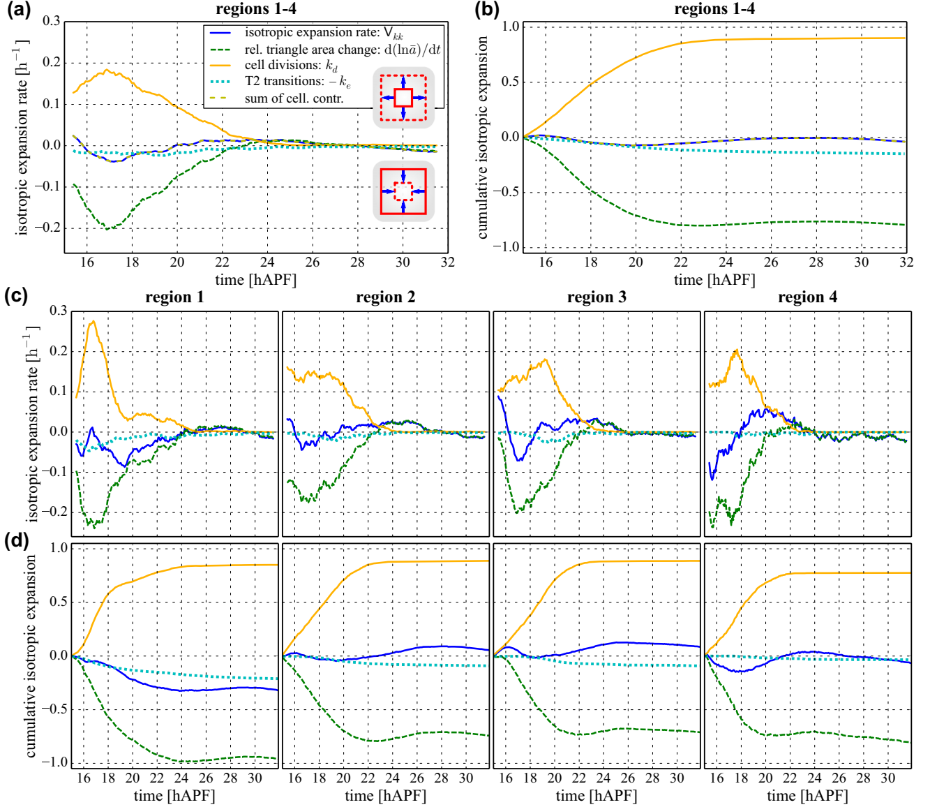
FIG. 12. Contributions to isotropic tissue expansion as a function of time during pupal development of the fly wing. Shown are the data for one wing. (a) Large-scale isotropic expansion rate and cellular contributions to it averaged over regions 1–4 as a function of time. (b) Cumulative isotropic expansion rate and cellular contributions to it. (c), (d) Same plots as in (a) and (b), but for the subregions 1 to 4 indicated in Fig. 11(a). The legend in (a) applies to (b)–(d), too. In all panels, data were averaged over 10 subsequent interframe intervals.
