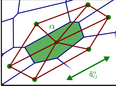
FIG. 6. The elongation \tilde{q}_{ij}^\alpha of a cell \alpha (green) is defined by the average elongation of the triangles belonging to \alpha (red). The triangles belonging to \alpha are those that have one of their corners defined by the center of \alpha .
