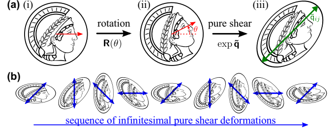
FIG. 15. Illustration of the shear-induced rotation effect \delta\xi appearing in Eq. (A22). For clarity, we use a Minerva head in place of a triangle. (a) The definitions of orientation angle \theta and elongation tensor \tilde{q}_{ij} are analogous to the triangle quantities [Fig. 4(c)]. Roughly, the orientation angle \theta corresponds to the direction in which the Minerva head looks. The isotropic scaling has been set to one for simplicity ( a = a_0 ). (b) The elongated Minerva head is subject to a continuous pure shear deformation with varying shear axis. The pure shear axis is at each time point oriented with an angle of \pi/4 with respect to the elongation axis \phi , such that the elongation norm |\tilde{q}| does not change but only the angle \phi . Here, snapshots of such a deformation are shown. Alternatively, Movie M5 shows this deformation more smoothly [30]. Strikingly, the head orientation angle \theta changes by this deformation although the deformation never includes any rotation component \delta\psi = 0 . Here, we have set |\tilde{q}| = (\ln 2)/2 such that \delta\theta = \delta\xi = 0.2\delta\phi .
