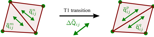
FIG. 8. A T1 transition induces an instantaneous change of the average triangle elongation. The average triangle elongation before and after the T1 transition only depends on the position of the four involved cell centers (green dots).
