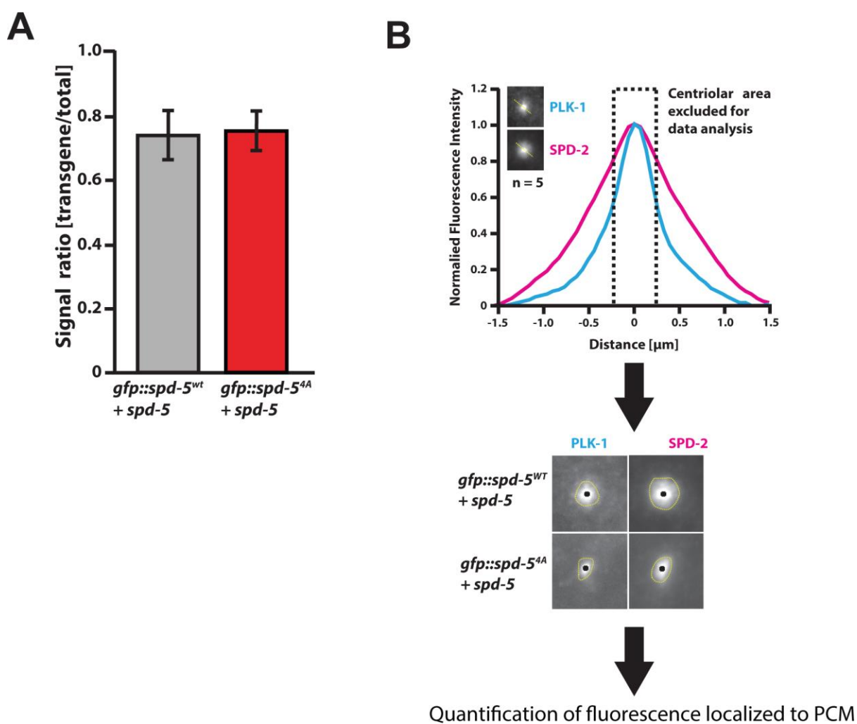
Fig. S2. Estimation of protein levels at the centrosome from immunostainings
