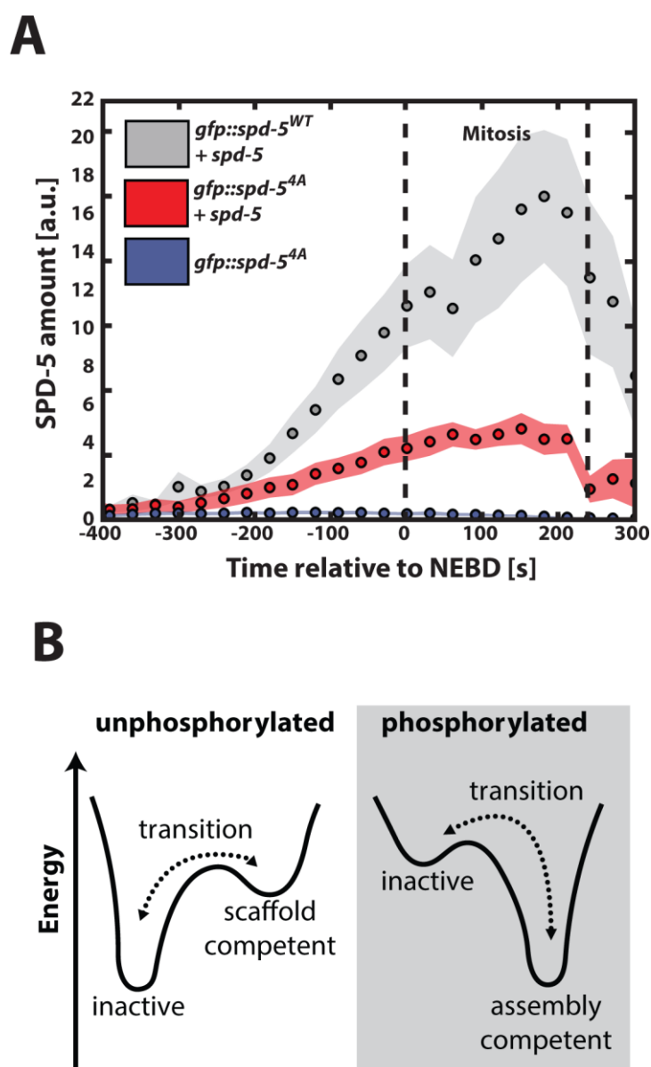
Fig. S3. Data and concept used to generate and test the theoretical model
