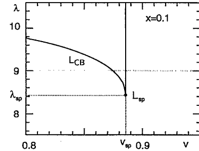
FIG. 9. Phase diagram as a function of the line tension \lambda and reduced volume v for fixed relative domain size x = 0.1 . For decreasing v , budding occurs continuously at L_{sp} , which is a stationary limit shape consisting of two spheres. At L_{CB} , the neck opens again. Budding does not occur for \lambda < \lambda_{sp} . The dotted line for \lambda = 9 corresponds to the sequence of shapes as shown in Fig. 8(b).
