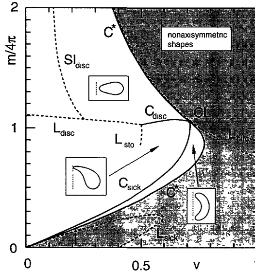
Fig.5. — Phase diagram for toroidal vesicles in the BC model. Three axisymmetric regions which are separated by continuous shape transformation lines C_{\text{sick}} and C_{\text{disc}} can be distinguished: i) discoid tori; ii) sickle-shaped tori and iii) toroidal stomatocytes. The line C^* indicates the instability with respect to axisymmetry breaking conformal transformations. On the right hand side of this line, non-axisymmetric shapes have minimal energy. The lines L_{\text{disc}} , L_{\text{sto}} and L_{\text{sick}} represent limit shapes with vanishing hole diameter. Above the line of circular limit shapes L_{\text{circ}} , no axisymmetric stationary shapes exist. The contour of discoid tori begins to selfintersect at the line SI_{\text{disc}} .
