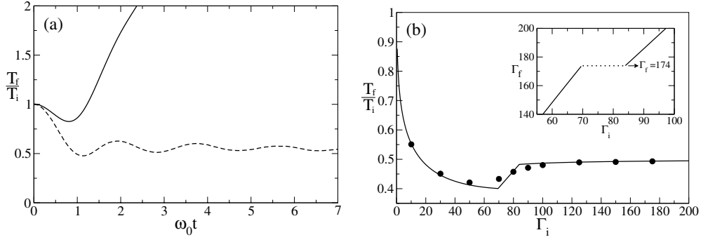
Figure 1. (a) Time evolution of the ionic kinetic energy, for the whole plasma cloud (solid) and for the central region only (dashed). (b) Ratio of final to initial temperature as a function of the density-scaled inverse initial ion temperature \Gamma_i , from the numerical simulations (full circles) and from equation (6) (solid line). The inset shows the final Coulomb coupling parameter.
