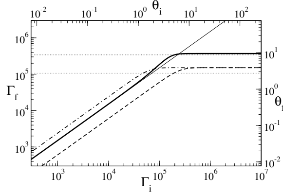
Figure 3. Final scaled temperature as a function of the initial scaled temperature for r_s = 2 \times 10^9 and for \omega_L/\omega_0 = 1 (thick solid line), \omega_L/\omega_0 = 2 (dashed line) and \omega_L/\omega_0 = 1/2 (dot-dashed line). For comparison, the result obtained with the classical expressions for initial- and final-state energies is shown by the thin solid line. The horizontal dotted lines show the estimate equation (11) for the limiting temperature.
