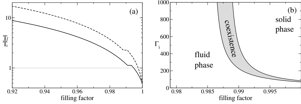
Figure 2. (a) Final temperature as a function of the lattice filling factor for \Gamma_i = 200 (solid line) and \Gamma_i = 400 (dashed line). The grey horizontal line separates cooling from heating. (b) Phase diagram for the final plasma state in the f - \Gamma_i plane.
