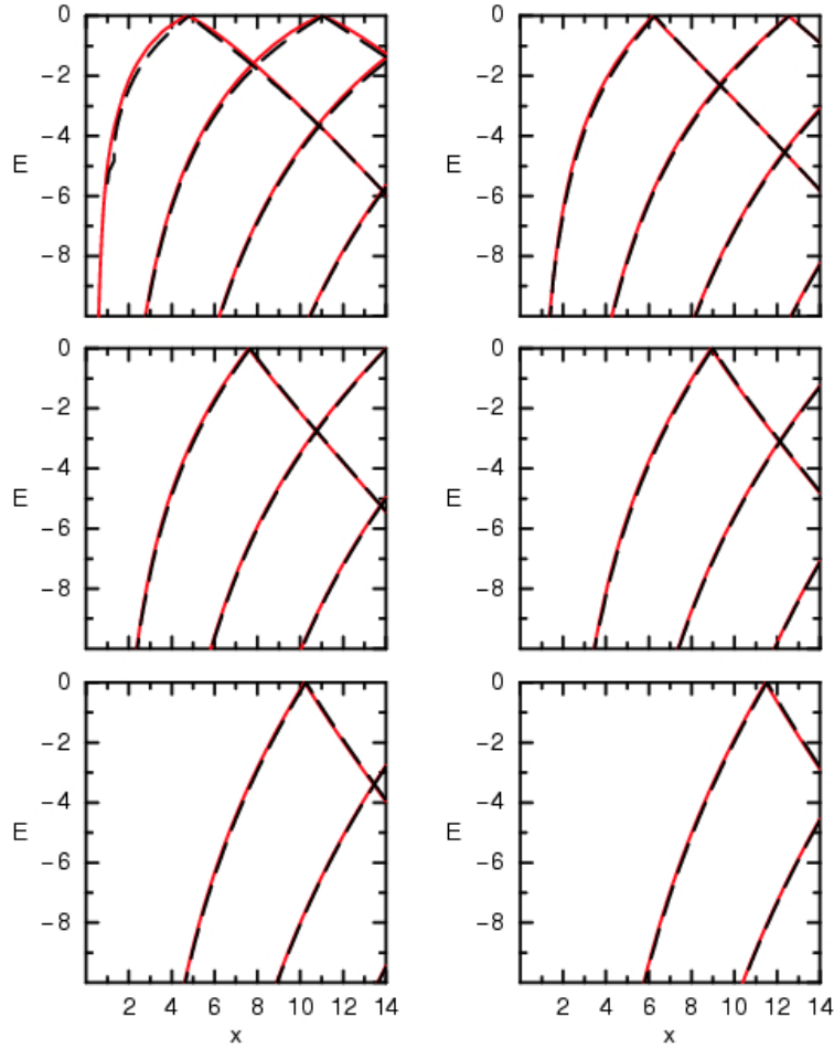
Figure 6: For the first six values of n , the graphical solution of the simultaneous equations (53) and (55) can be read off from the intersections of the gray curves. The dashed black curves show the analogous graphical solution of Eqs. (29) and (31). The exact and semiclassical curves are almost indistinguishable (except for n = 0 ), attesting to the striking accuracy of the former even at the smallest possible size parameters x . All plots can be continued to Z > 0 by reflecting at the axis Z = 0 . The WKB curves with positive slope belong to Eq. (55), the falling lines are created by Eq. (53). They are labeled starting from the leftmost by \mu, \nu = 0, 1, 2 \dots
