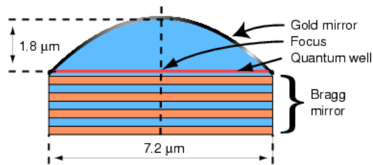
Figure 2: Schematic cross-section of a semiconfocal parabolic dome cavity, consisting of parabolic gold mirror and a planar Bragg mirror placed at the focal plane of the parabola. The cavity spacer is made of GaAs, and the light emitter is a quantum well placed in the vicinity of the focal plane.
