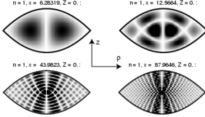
Figure 7: Four states with n = 1 . Gray scale indicates the magnitude of the electric field for the modes ( E_{\pm} ) of the confocal double paraboloid, highest fields shown in black. The vertical axis is z , the horizontal axis the axial distance \rho . Increasing x means shorter wavelength and hence more nodal lines (white). The size parameter is quantized according to Eq. (56) with N = 1, 2 in the top row, and N = 7, 14 at the bottom.
