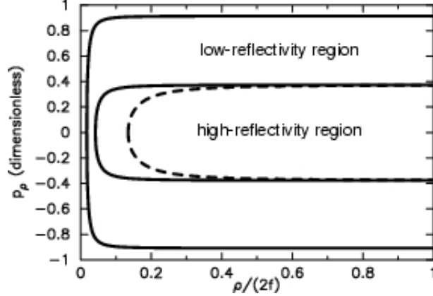
Figure 16: Assuming that the Bragg mirror stack at the plane z = 0 yields high reflectivity only for waves within \chi_c = 22^\circ from the surface normal or for, the regions of high reflectivity in the Poincaré section are bounded by Eq. (96). The resulting curves bounded by |p_\rho| < 0.374 are shown for L_z = 0.03 (solid line) and L_z = 0.1 (dashed). A second high-reflectivity window exists for rays falling between the boundary of this plot and the solid line near the boundary. It becomes relevant only for the integrable confocal cavity because the perturbed shapes have no stable orbits in this second window.
