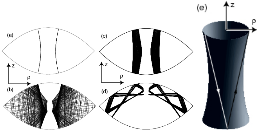
Figure 13: Trajectories in the non-confocal cavity. (a) shows the unstable periodic orbit arising at \epsilon = 0.02 f , L_z = 0.1 f , cf. Fig. 12. For the same parameter, a chaotic trajectory is seen in (b). Oscillatory motion around stable periodic orbits occurs in (c) and (d), where \epsilon = -0.02 f and L_z = 0.1 f as in the SOS of Fig. 14. The patterns of type (a) and (c) derive from the periodic motion of Fig. 10 (a) as a result of the shape perturbation. In real three-dimensional Cartesian space, (e) shows the straight-line ray motion (arrows) giving rise to the curved “envelope” surface whose cross section we see in (a).
