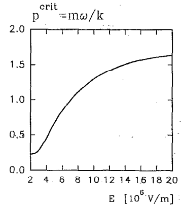
FIG. 12. The minimal critical value of transfer momentum p = m\omega/k , below which no plasma oscillation occurs vs electric field.
