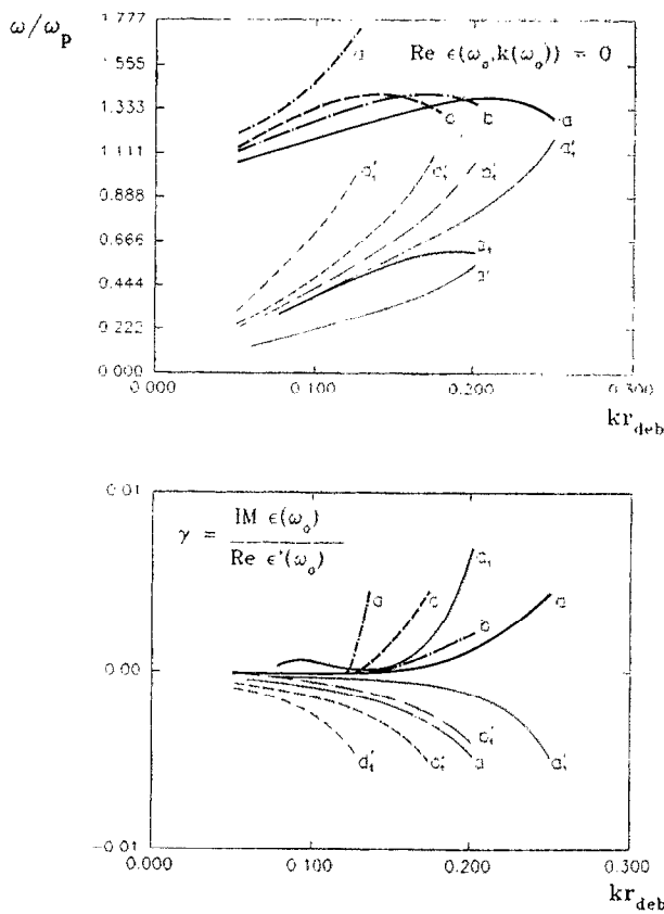
FIG. 9. The plasma oscillation dispersion (above) for four different field strengths vs wave vector together with the corresponding increment. The letters a-d stand for the field strengths: 5 \cdot 10^6 V/m, 6 \cdot 10^6 V/m, 7 \cdot 10^6 V/m, 1 \cdot 10^7 V/m. The prime indicates the acoustic modes and the subscript 0.1 labels the doubled mode by the field.
