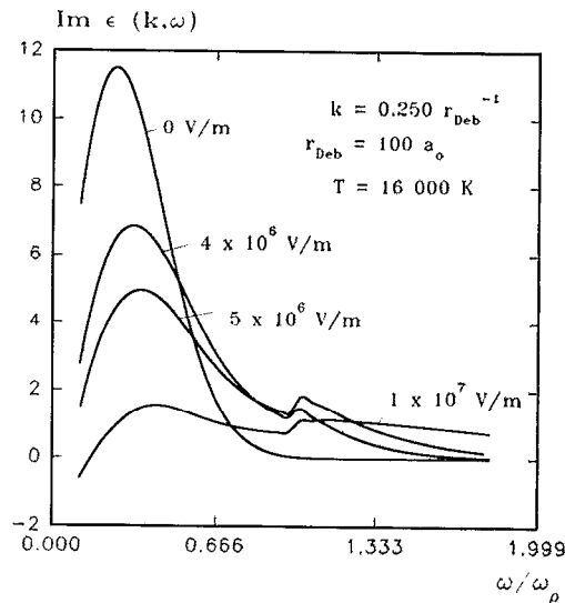
FIG. 5. The imaginary part of the DF of one momentum of k=0.25 \hbar r_{\text{Deb}}^{-1} vs frequency for the case of four different field strengths and a temperature of 16 000 K and an electron density of 10^{18.1} , which corresponds to the situation of the distribution functions in Fig. 1.
