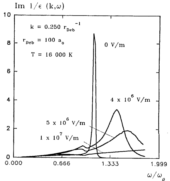
FIG. 6. The excitation spectra of the DF of one momentum of k=0.25 \hbar r_{\text{Deb}}^{-1} vs frequency for the case of four different field strength and a temperature of 16 000 K and an electron density of 10^{18.1} , which corresponds to the situation of the distribution functions in Fig. 1.
