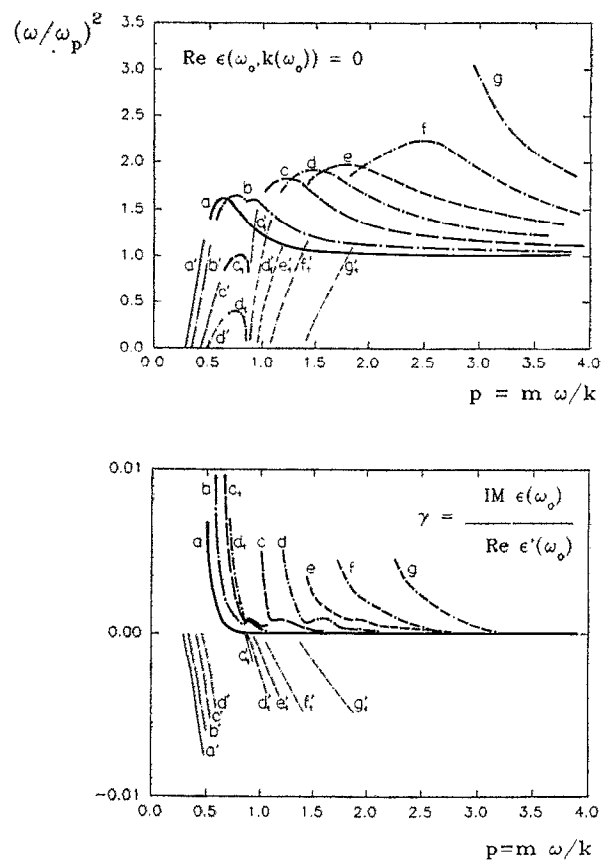
FIG. 10. The plasma oscillation dispersion (above) for seven different field strengths vs transfer momentum together with the corresponding increment. The letters a-g stand for the field strengths: 0 V/m, 2 \cdot 10^6 V/m, 4 \cdot 10^6 V/m, 5 \cdot 10^6 V/m, 6 \cdot 10^6 V/m, 7 \cdot 10^6 V/m, 1 \cdot 10^7 V/m. The prime indicates the acoustic modes and the subscript 0.1 labels the doubled mode by the field.
