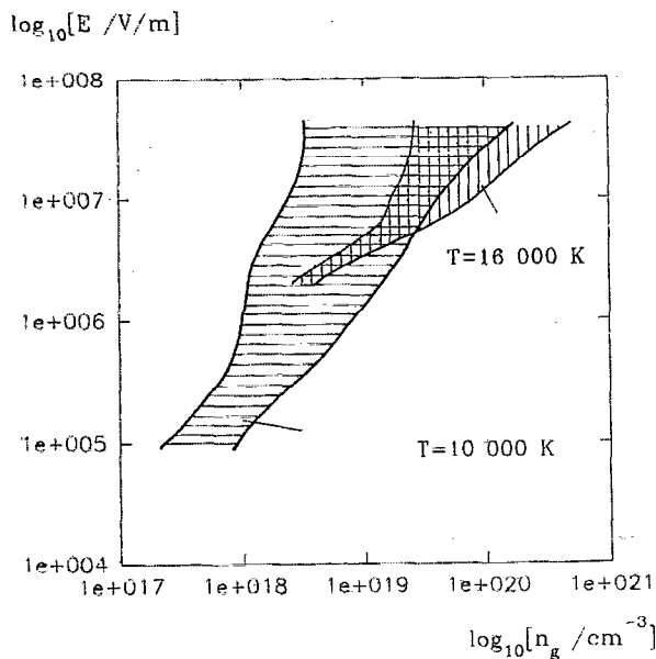
FIG. 7. The electric field-total electron density plane, where plasma instabilities can occur following Penrose for two different temperatures. The temperature of 16 000 K corresponds to the situation calculated in Fig. 1.
