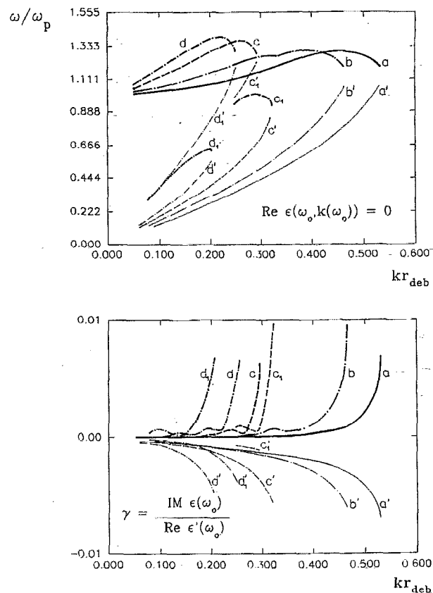
FIG. 8. The plasma oscillation dispersion (above) for four different field strengths vs wave vector together with the corresponding increment (below). Different branches are signed with different lines belonging to the upper ones. The letters a-d stand for the field strengths: 0 V/m, 2 \cdot 10^6 V/m, 4 \cdot 10^6 V/m, 5 \cdot 10^6 V/m. The prime indicates the acoustic modes and the subscript 0.1 labels the doubled mode by the field.
