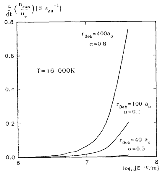
FIG. 2. The runaway electron stream in % of the electron density per atomic time units vs electric fields for different screening parameters in the partially ionized hydrogen plasma and a temperature of 16 000 K.
