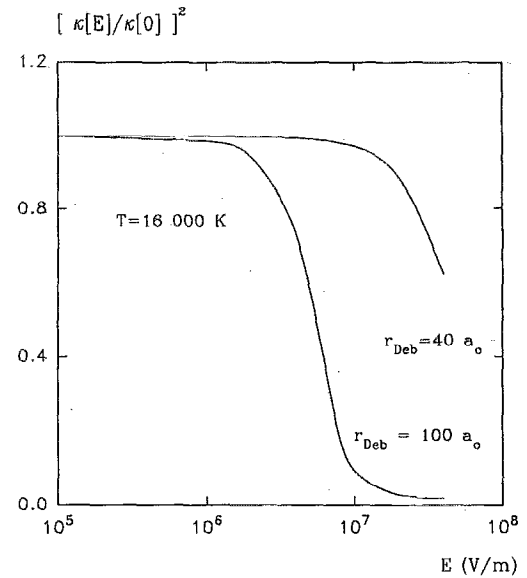
FIG. 3. The ratio of field-dependent Debye-screening parameters to field-free one vs field strength, a temperature of 16 000 K and two different Debye lengths.
