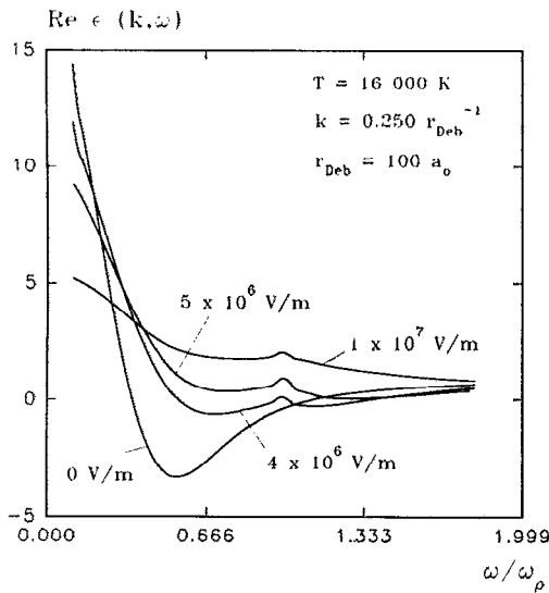
FIG. 4. The real part of the DF for one momentum of k=0.25 \hbar r_{\text{Deb}}^{-1} ( r_{\text{Deb}} Debye radius) vs frequency for the case of four different field strengths, a temperature of 16 000 K and an electron density of 10^{18.1} , which corresponds to the situation of the distribution functions in Fig. 1.
