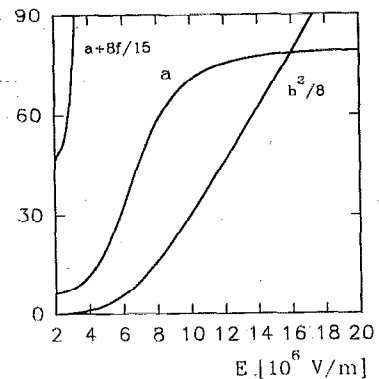
FIG. 13. The two constants of mean kinetic energy a and the mean stream energy b , which decide, whether plasma oscillations occur, vs electric fields.
