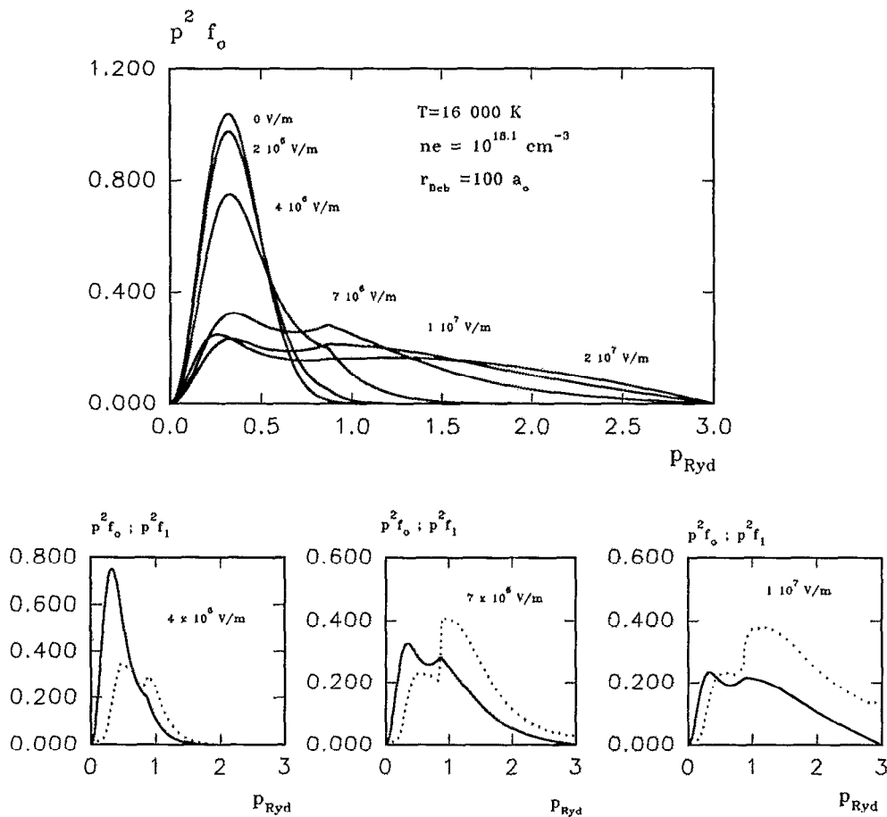
FIG. 1. Isotropic distribution function (above) in artificial units vs momentum for a free electron density of 10^{18.1} \text{ cm}^{-3} , an ionization degree of 0.1 and a temperature of 16 000 K with six different field strengths. The corresponding Debye-radius is r_{\text{Deb}} = 100 a_0 , with a_0 the atomic radius. In the below 3 fields are picked out together with the corresponding anisotropic part (dotted line).
