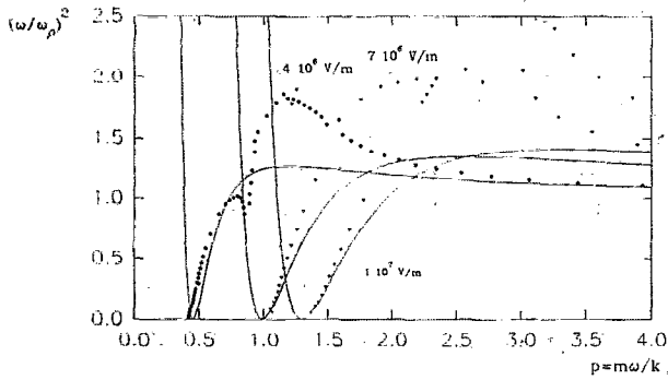
FIG. 11. The plasma oscillation dispersion for three different field strengths vs transfer momentum together with the linearized model.
