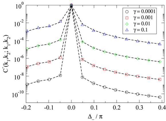
Fig. 5. Weight function for different values of the interaction strength \gamma of the eigenstate \nu = 145 along the \Delta_- direction. The dashed lines are results from formula (24). Here f = 40 .
