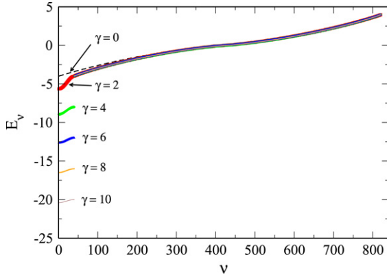
Fig. 1. Energy spectrum of the two-boson BH chain with fixed boundary conditions for different values of the interaction strength \gamma . The eigenvalues are plotted as a function of the eigenvalue label (see text). Here f = 40 .
