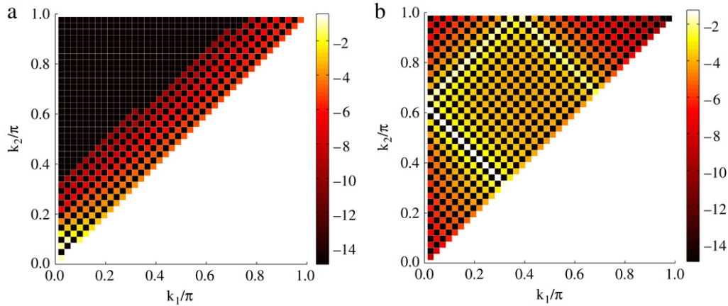
Fig. 9. 3-D plot of the logarithm of the weight function in normal-mode space for the eigenstate \nu = 25 , that belongs to the two-boson bound state band. Results were obtained by numerical diagonalization. (a) \gamma = 1.5 . The two-boson bound state band did not split off and the eigenstate is localized in normal-mode space. (b) \gamma = 2 . At this interaction value the two-boson bound state band splits off and the eigenstate becomes delocalized in normal-mode space. Here f = 8 .
