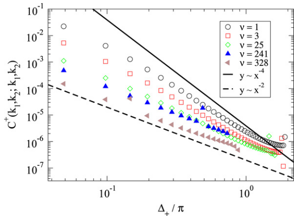
Fig. 6. Weight function of different eigenstates (labeled by the index \nu ) along the \Delta_+ direction. Here \gamma = 0.1 and f = 40 .
