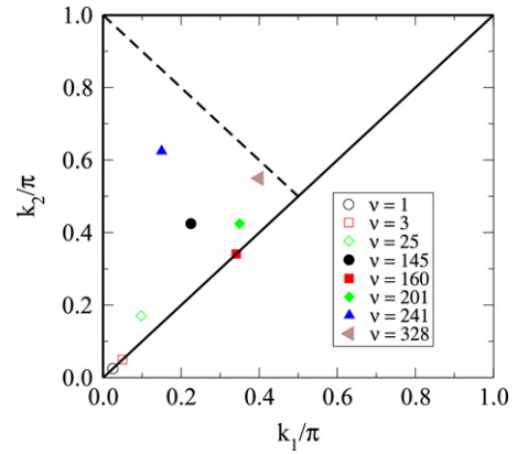
Fig. 8. Location P = (\hat{k}_1, \hat{k}_2) of the eigenstates, shown in Figs. 6 and 7, in the irreducible triangle.
