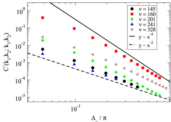
Fig. 7. Weight function of different eigenstates (labeled by the index \nu ) along the \Delta_- direction. Here \gamma = 0.1 and f = 40 .
