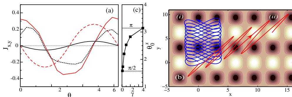
FIG. 1 (color online). (a) Dependence of the current components, J_x (solid line) and J_y (dashed line), on \theta for (1), (10), and (11) with D = 1 , E_x^{(1)} = -E_x^{(2)} = 2 , E_y^{(1)} = -E_y^{(2)} = 2.5 . Data are for the overdamped ( \mu = 0 , \gamma = 1 thick lines) and underdamped ( \mu = 1 , \gamma = 0.1 thin lines) cases, respectively; (b) the time evolution of the mean particle position, \bar{\mathbf{r}}(t) = \int \mathbf{r} P(\mathbf{r}, \mathbf{v}, t) d\mathbf{r} d\mathbf{v} , for \theta = 0 . The trajectories are superimposed on the contour plot of the potential (10). Curve (i) corresponds to E_x^{(1)} = 3 , E_x^{(2)} = E_y^{(1)} = 0 , E_y^{(2)} = 3.5 and curve (ii)—to the parameters of panel (a). The other parameters are D = \mu = 1 , \gamma = 0.1 ; (c) the phase lag \theta_x^{(0)} as a function of the dissipation strength \gamma .
