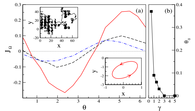
FIG. 2 (color online). (a) Dependence J_\Omega(\theta) , Eq. (12), for (1), (16), and (17), with \mu = 1 , D = 0.5 , E_x^{(1)} = 0.4 , E_y^{(1)} = 0.8 and \gamma = 0.2 (solid line), \gamma = 0.05 (dashed line), and \gamma = 2 (dash-dotted line). Insets: the trajectory (left inset) and the corresponding attractor solution, \bar{\mathbf{r}}(t) , (right inset) for the case \gamma = 0.2 and \theta = \pi/2 . We have used N = 10^5 independent stochastic realizations to perform the noise averaging; (b) the phase lag \theta_0 as a function of the dissipation strength \gamma .
