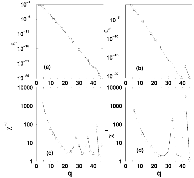
FIG. 3. Parameters: N=47 , \alpha=0.1 , \mathcal{E}=0.0025 . (a) Energy of normal modes vs mode number of a QB for q_0=2 . (b) Similar to (a), but for a QB with q_0=3 . (c) Sequence \chi_j^{-1} for q_0=2 . (d) Sequence \chi_j^{-1} for q_0=3 .
