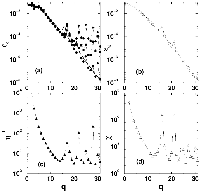
FIG. 1. (a) Natural packet evolution initially exciting mode q_0=1 . The energies of normal modes are plotted vs q . (Circles) 10^4 , (squares) 10^5 , (rhombs) 10^6 . (Dashed line) q -breather from (b) for comparison. (b) The energies of normal modes vs q for a q -breather with q_0=1 . (c) Sequence \eta_j^{-1} . (d) Sequence \chi_j^{-1} . Parameters in all cases: N=31 , \alpha=0.33 , \mathcal{E}=0.01 .
