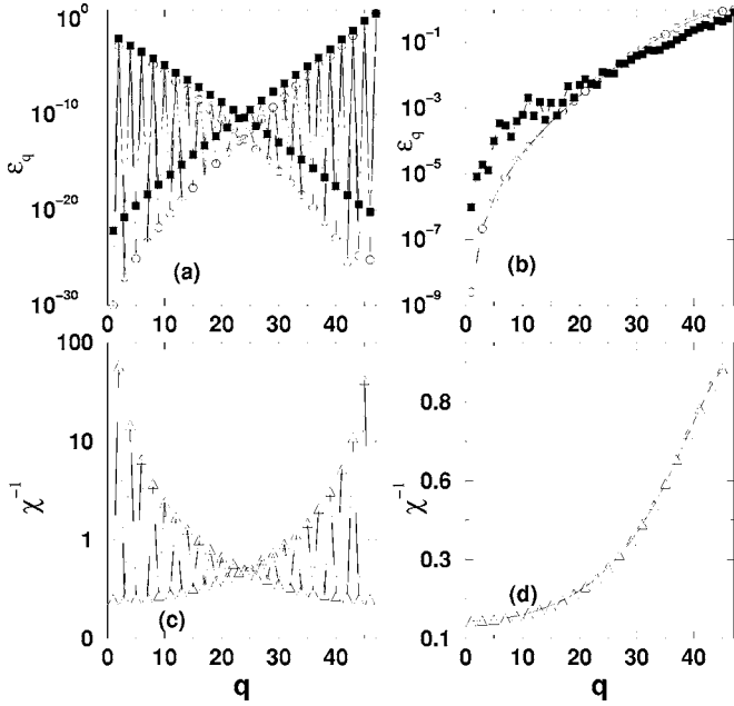
FIG. 4. Parameters: N=47 , \mathcal{E}=0.1 . (a) Energy of normal modes in a QB (open symbols) and a natural packet (filled symbols, waiting time 10^5 ) for q_0=47 and \alpha=0.25 . (b) Similar to (a), but for \beta=0.25 . (c) Sequence \chi_j^{-1} , which corresponds to case (a). (d) Sequence \chi_j^{-1} , which corresponds to (b).
