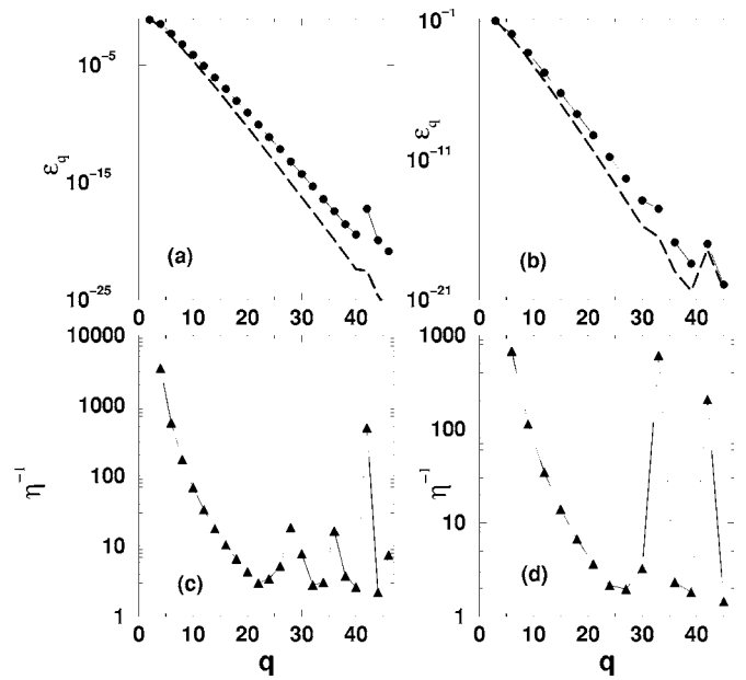
FIG. 2. (a) Natural packet evolution initially exciting mode q_0=2 (circles). The energies of normal modes are plotted vs q at t=10^5 . The dashed line shows the energy distribution for a corresponding q -breather with q_0=2 . (b) Same as (a), but for q_0=3 . (c) Sequence \eta_j^{-1} for q_0=2 . (d) Sequence \eta_j^{-1} for q_0=3 . Parameters in all cases: N=47 , \alpha=0.1 , \mathcal{E}=0.0025 .
