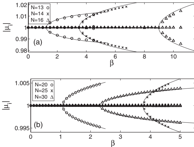
FIG. 3. Absolute values of Floquet eigenvalues (symbols) and analytical curves (solid lines) for QBs with E_{\text{tot}} = 1.5 and (a) \mathbf{q}_0 = (3, 3) , N = 13, 14, 16 [the instabilities correspond to \mathbf{k} = (1, 2) and \mathbf{k} = (2, 1) ] and (b) \mathbf{q}_0 = (2, 3) , N = 20, 25, 30 [the instabilities correspond to \mathbf{k} = (1, 1) for N = 20, 25 and \mathbf{k} = (1, 2) for N = 30 ].
