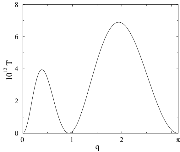
FIG. 2. Transmission coefficient versus q for a Klein-Gordon chain breather with \Omega_b = 1.38 and C = 0.001 .
