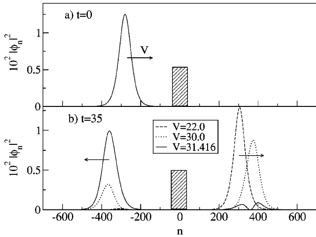
FIG. 3. Profiles of the wave field in the initial state (a) and after the interaction (b). The Fano defect (marked by the shaded bar) is placed at n=0 , and the direction of motion of the pulses is indicated by arrows. The parameters are: E=0 (i.e., q_F = \pi/2 ), C=10.0 , and \epsilon=4.0 , \eta=\lambda=1.0 . After the interaction, two soliton-like pulses are observed, which move in the opposite directions with equal absolute values of their velocities.
