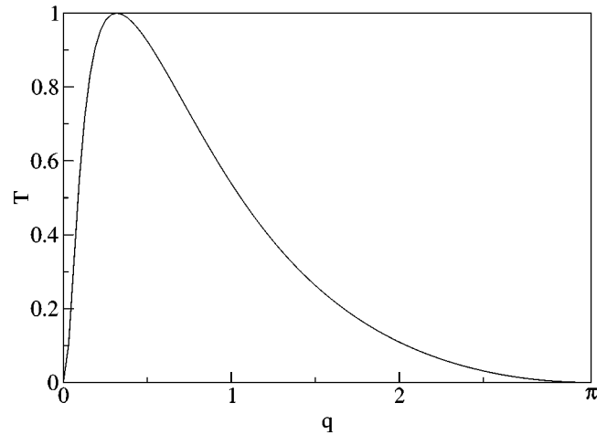
FIG. 1. The transmission coefficient T vs q for the case of the resonant transmission, as per Eq. (3) with C=10 and \epsilon=19 .
