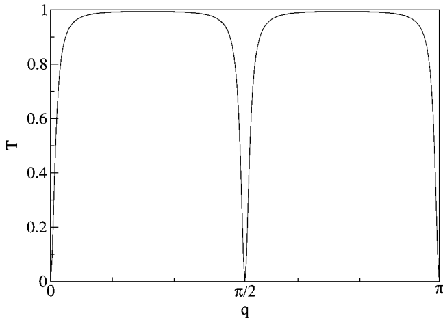
FIG. 2. The transmission coefficient as given by Eq. (8), versus the wave number q of the incident wave. The parameters are E=0 , C=10 (i.e., q_F = \pi/2 ), and \epsilon=4 .
