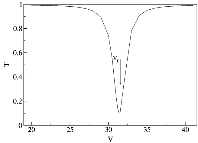
FIG. 4. The transmission coefficient for the scattering of the soliton on the Fano defect, defined as in Eq. (9) and found from direct simulations, vs the soliton's velocity V . Parameters are the same as in Fig. 2. The minimum is located at V_F = 2Cq_F .
