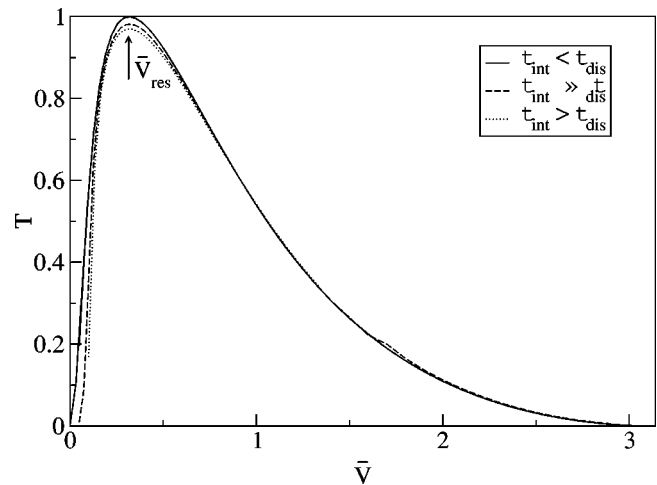
FIG. 6. A typical dependence of the transmission coefficient T for the soliton in the model (11) on V for \eta = \lambda = 1 and (a) \epsilon = 19 and C = 10 (solid line); (b) \epsilon = 3.8 and C = 2 (dashed line); (c) \epsilon = 2.85 and C = 1.5 (dotted line). In this figure, the normalized velocity V = V/2C is used. In all the cases, the position of the resonance is fixed at \bar{V}_{\text{res}} \approx 0.318 .
