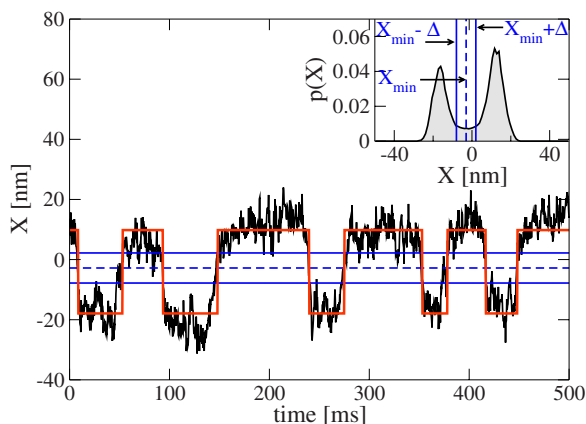
FIG. 2. (Color online) Binary-filtering of the hair bundle's trajectory. A sample trajectory X(t) of a spontaneous hair bundle oscillation and its discretization is depicted. The inset shows the probability distribution p(X) for spontaneous oscillations. In order to discretize the trajectory we implemented a two-threshold criterion where the trajectory has to cross a state-dependent threshold. The minimum X_{min} of the probability distribution for X serves as an indicator at which position X a transition occurs. There the trajectory spends the least time because it is fast and therefore the probability is reduced. The two thresholds are placed symmetrically about the minimum X_{min} \pm \Delta . The discretization procedure is then as follows: being in state \sigma_- , X(t) needs to cross the threshold X_{min} + \Delta to detect a transition. Being in state \sigma_+ , the threshold is set to X_{min} - \Delta . We chose \Delta = 5 nm throughout this paper. The discretization thresholds X_{min} \pm \Delta are indicated in the figure. The peak-to-peak amplitude \sigma_+ - \sigma_- of the binary trajectory was adjusted such that the variances of the two processes are equal.
