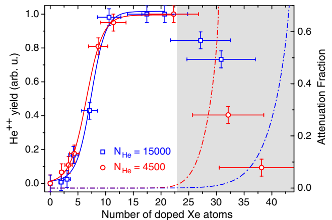
FIG. 2 (color online). Xe doping dependence of He ^{++} yields at a peak laser intensity of 1.5 \times 10^{14} W/cm ^2 for droplets with a mean number of He atoms per droplet N_{He} = 4500 (red) and N_{He} = 15000 (blue). Horizontal bars present the error in estimating the number of doped Xe atoms. The dash-dotted curves present the fraction of droplets lost due to complete evaporation, which is significant only for numbers of Xe dopant atoms K \geq 20 (gray shading).
