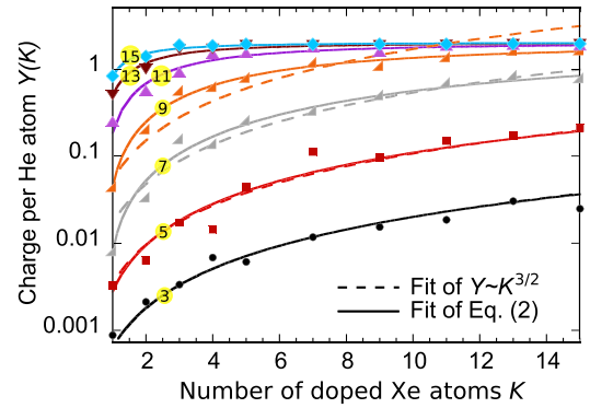
FIG. 4 (color online). Average charge per He atom Y(K) as a function of the number of doped Xe atoms for a droplet with 4000 He atoms and intensity as in Fig. 1 from molecular dynamics calculations. The curves correspond to different laser pulse lengths (full width at half maximum): from 3 (bottom) to 15 fs (top) in steps of 2 fs, as shown in the labels. The lines are fits of the data points according to Eq. (2) (solid line) and with the power law Y \propto K^{3/2} corresponding to ionization by a static field for T \leq 9 fs (dashed line). For details, see the text.
