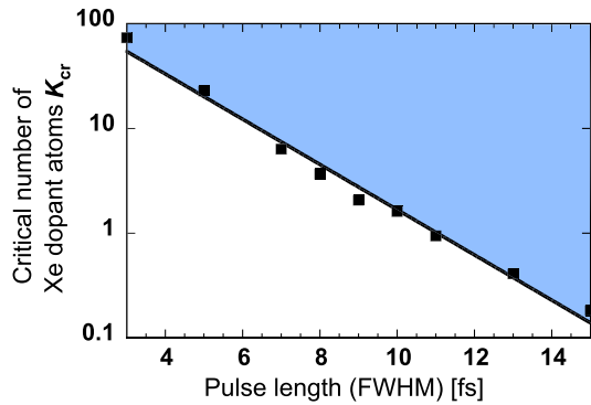
FIG. 5 (color online). The number of dopants for which the average charge per He atom Y in Fig. 4 has a turning point: Y''(K_{\text{cr}}) = 0 . The shaded area distinguishes the regime of DII from the field ionization regime (not shaded), at a peak intensity of 7 \times 10^{14} W/cm 2 .
