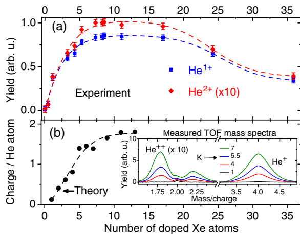
FIG. 1 (color online). (a) Yields of He ^{++} and He ^+ ions as a function of the mean number of Xe dopants in a nanodroplet containing 1.5 \times 10^4 He atoms at a peak laser intensity of 7 \times 10^{14} W/cm ^2 . (b) Numerical calculation of the charge per He atom as a function of the number of Xe atoms in a droplet containing 4000 He atoms. All lines are to guide the eye. Inset: Time-of-flight mass spectra of He ^{++} and He ^+ ions for different numbers of dopant Xe atoms ( K ) as shown in the legend.
