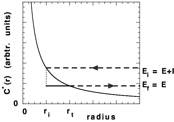
FIG. 1. Sketch of tunneling threshold dynamics on the fixed point manifold with potential C_*(r) from Eq. (7). The classically allowed incoming and outgoing trajectory on the respective energies E_i and E_f is shown (dashed lines) as well as the tunneling part (solid thick line) which determines the threshold fragmentation probability.
