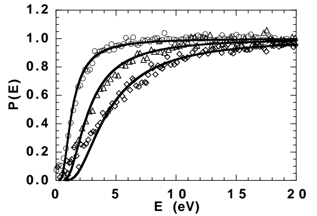
FIG. 2. Detachment cross section by electron impact as a function of excess energy for B^- (circles) from [4], O^- (triangles) and D^- (diamonds) from [1]. The solid lines are the cross sections from Eq. (4).
