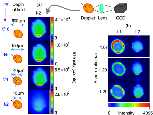
FIG. 4. (a) Images of broadly-pumped lasing prolate droplets ( b/a = 1.29 ) at \theta_D = 142^\circ with various f-numbers ( f/16 , f/8 , f/4 , and f/2 ). Because the solid angle of light acceptance is proportional to \approx 1/(f/\#)^2 , the color intensity scale for each f/\# is adjusted accordingly. The depth of field [ \propto (f/\#)^2 ] for each f/\# is shown relative to the droplet size. The imaging direction is on the right of the droplet. (b) Lasing images of broadly-pumped prolate droplets with various aspect ratios. Dynamical eclipsing is not present for small deformation ( b/a = 1.07 ).
