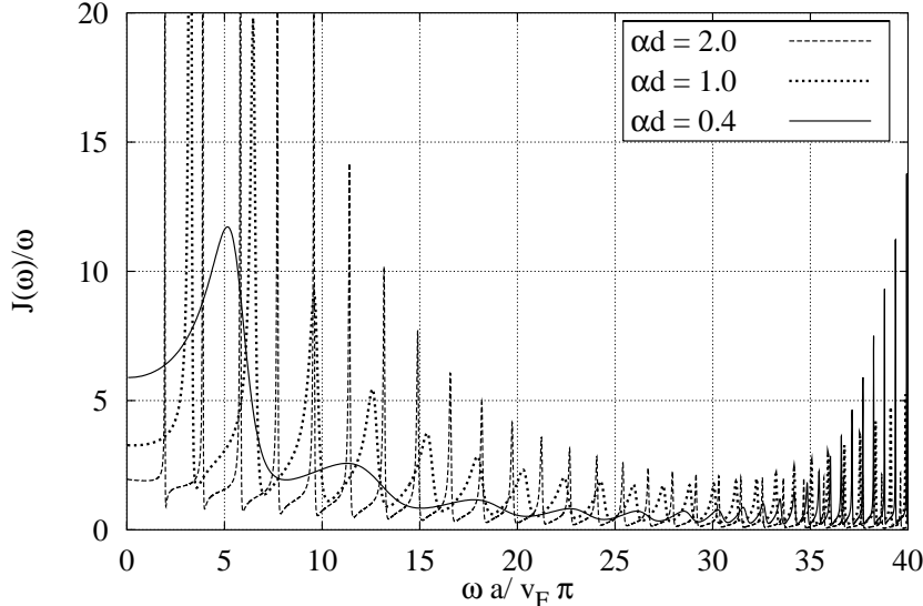
Figure 2: Spectral densities J(\omega)/\omega for the interaction V(x) = 2V_0/(\alpha d)^2 \exp(-\alpha|x|) as a function of normalized frequency \omega a/v_F\pi where a/d = 10\pi and g_0 = [1 + V_0/(\hbar\pi v_F)]^{-1/2} = 0.5 . The interaction range is tuned by \alpha d = 2, 1, 0.4 (increasing range).
