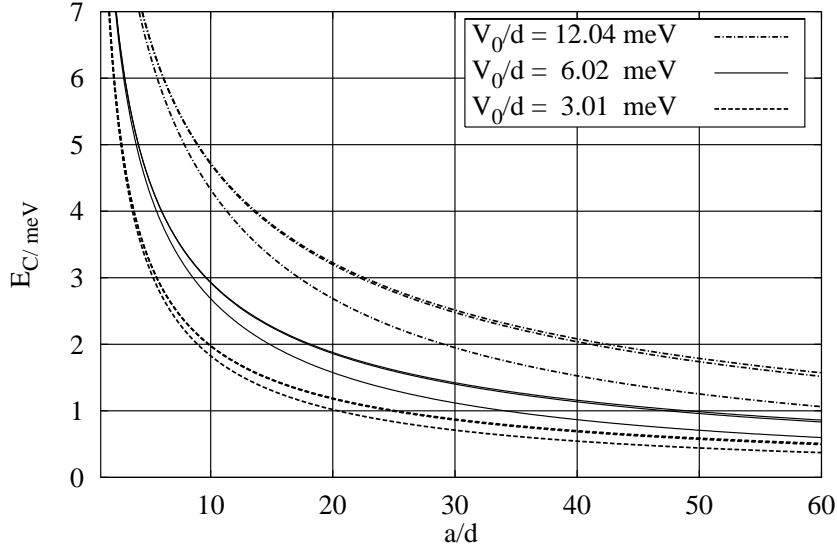
Figure 1: Charging energy E_\rho in meV as a function of a/d (Fermi energy E_F = 3 meV, effective electron mass m = 0.067m_0 ), d = 20 nm, interaction strengths V_0/d = 12.04 meV (dashed-dotted), 6.02 meV (full lines,) and 3.01 meV (dotted), corresponding to \epsilon = 3, 6, 12 , D/d = 500, 50, 5 (top to bottom).
