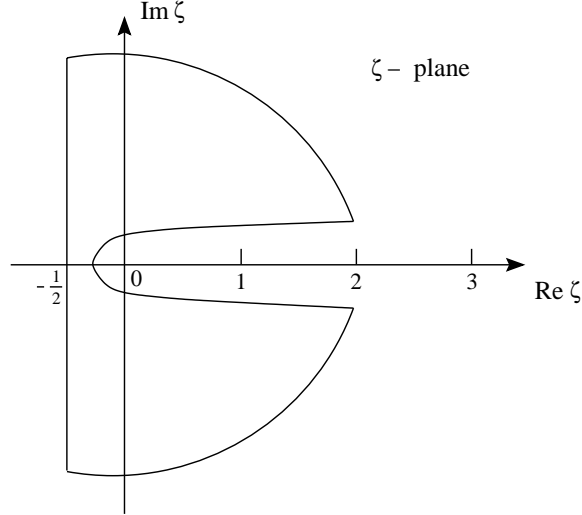
Fig. 2. Integration path for the evaluation of integral (65)
